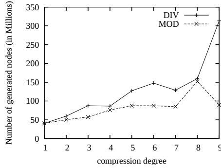
Figure 9: Nodes generated by DIV and MOD for the 9-token PDB of the (17,4)- Top-Spin problem
