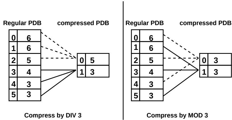
Figure 4: Compressed pattern database
