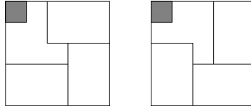
Figure 8: The 6-6-6-6 PDB for 24-Puzzle and its reflection
