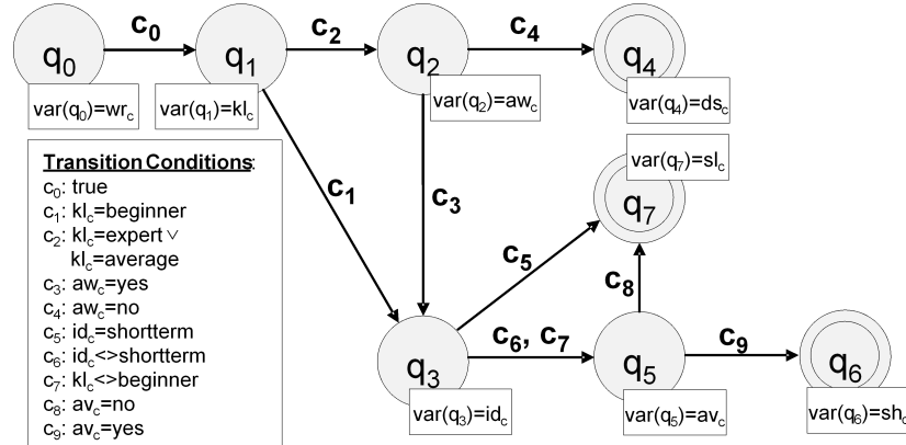
Fig. 1 Recommender user interface description: a simple example recommendation process for financial services. The process starts in state q_0 , and, depending on the user’s knowledge level, is forwarded to either state q_2 or state q_3 . In the final state (one of the states q_4, q_6, q_7 ) the recommended items are presented. Each state q_i has an assigned customer property var(q_i) that represents a question to be asked in this state.
