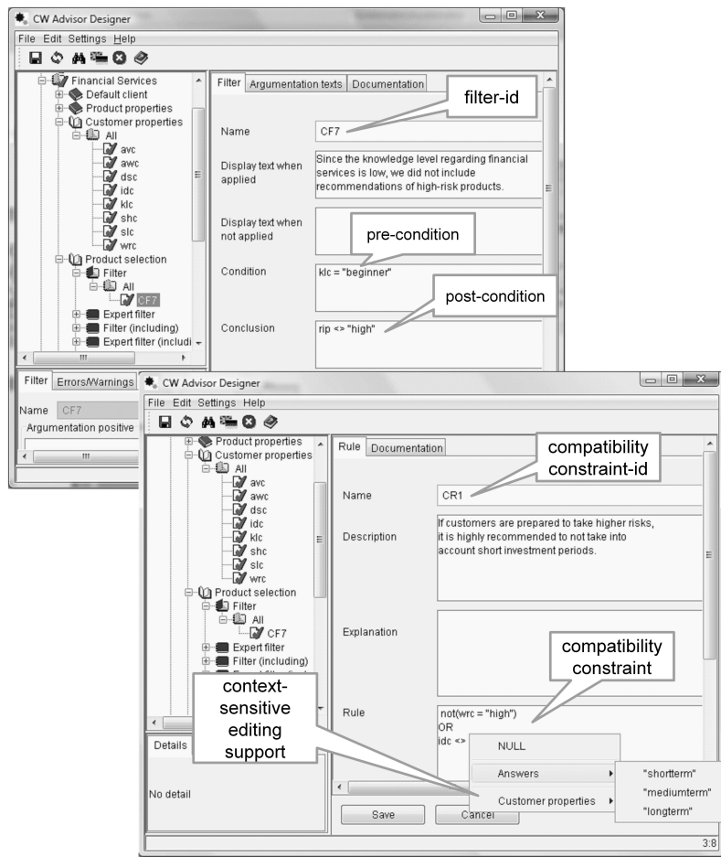
Fig. 2 CWAdvisor Designer Environment. Filter constraints (conditions) as well as compatibility constraints can be defined in a context-sensitive editing environment.
