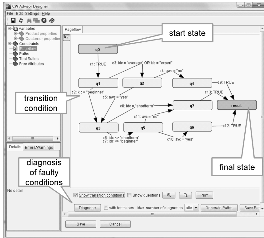
Fig. 3 CWAdvisor Designer Environment. Recommendation processes are specified on a graphical level and can be automatically translated into a corresponding executable representation. Faulty transition conditions can be identified automatically on the basis of model-based diagnosis [20].
