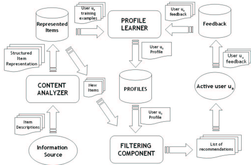
Fig. 1 High level architecture of a Content-based Recommender
